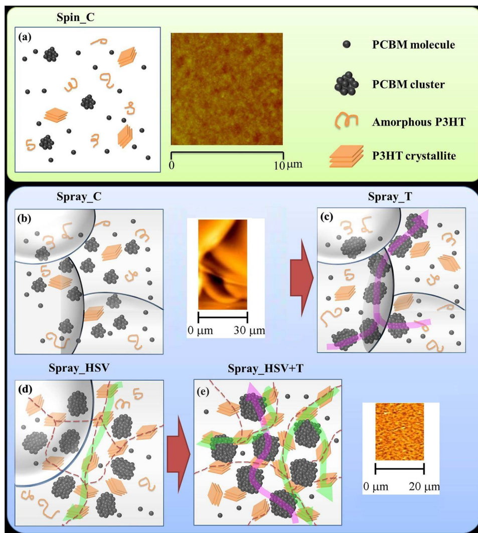
Figure 2. Schematics of the hierarchical BHJ structures controlled by various post-treatments: (a) Spin_C film with a low fraction of small PCBM clusters, (b) Spray_C film with a medium fraction of small PCBM clusters confined in the droplet boundaries, (c) Spray_T film with large aggregated PCBM clusters limited by the droplet boundaries (constructing into a PCBM network), (d) Spray_HSV film with few droplet boundaries and the network of P3HT crystallites formed with the elimination of the droplet boundaries. (e) Spray_HSV + T film with the interpenetrated networks formed by a large amount of P3HT crystallites and large PCBM clusters. The formation is closely related to the original droplet boundary. (a,b,e) include the representative AFM morphologies. These spray-coated BHJ structures reveal the mutual interaction between PCBM aggregation (nanoscale clusters) and P3HT crystallization confined in the droplet boundaries during phase separation. The hot solvent vapor and final thermal treatments eliminated the droplet boundaries and thus produced the related networks (as shown by dash lines) of P3HT crystallites or PCBM clusters. The favorable network paths for transporting electrons (purple arrow) and holes (green arrow) in the traverse direction were formed.
